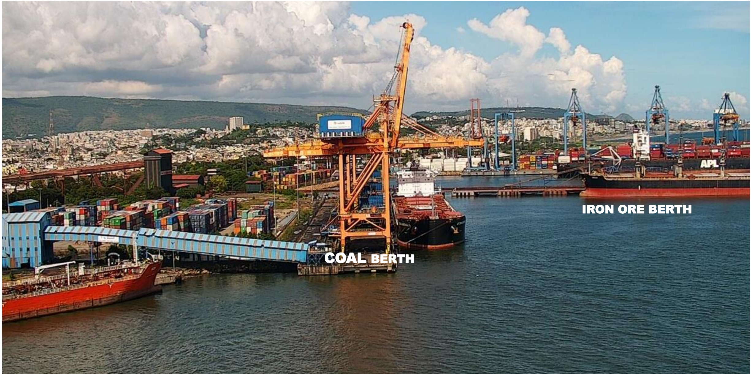
MECHANISED COAL AND IRON ORE HANDLING SYSTEMS WITH CLOSED CONVEYORS
